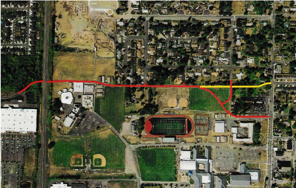
Figure 10. Alignment Options for NW 5 th Street
