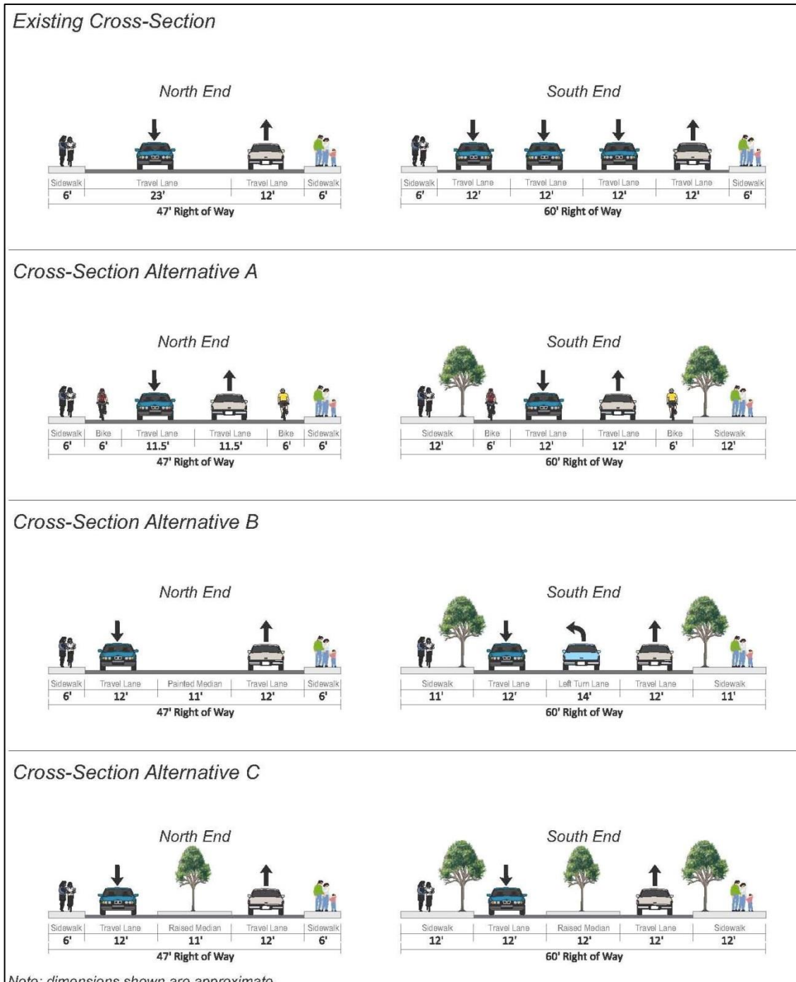
Figure 9. NW 12 th Avenue Cross-Section Alternatives (W Main Street to NW 1 st Street)
