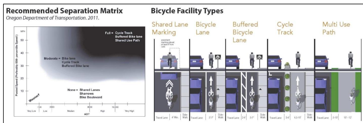
Figure 4. Bikeway Design Considerations
